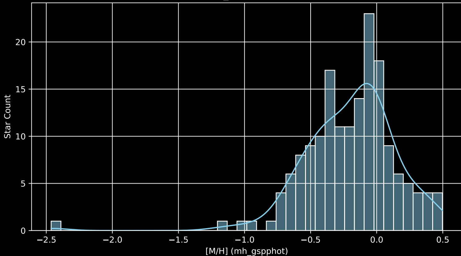
APOGEE DR17 Field: [273-24-O_TESS [M/H] (mh_gspphot) (n= 168)
