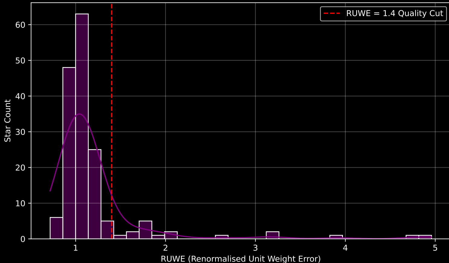
GAPOGEE DR17 Field [273-24-O_TESS] RUWE Distribution (n= 164)
