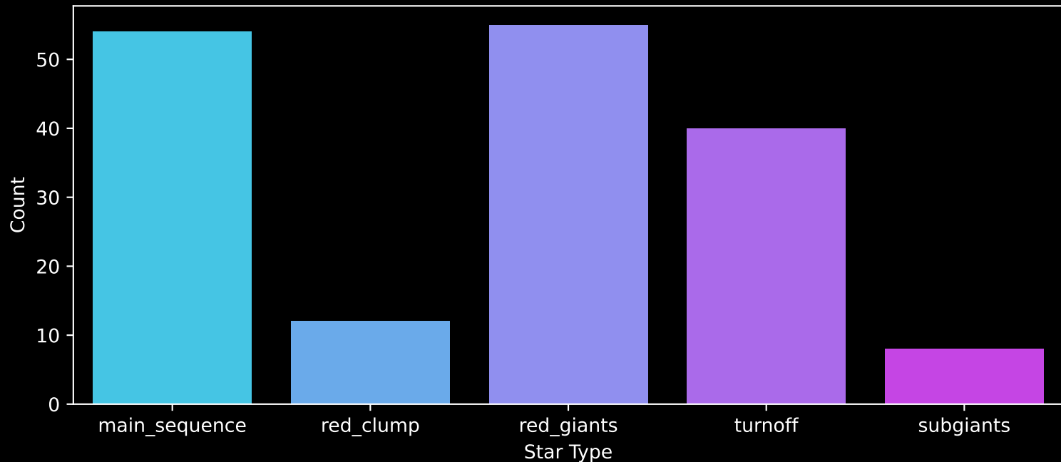
APOGEE DR17 Field: [273-24-O_TESS] Count plot of Star Type
