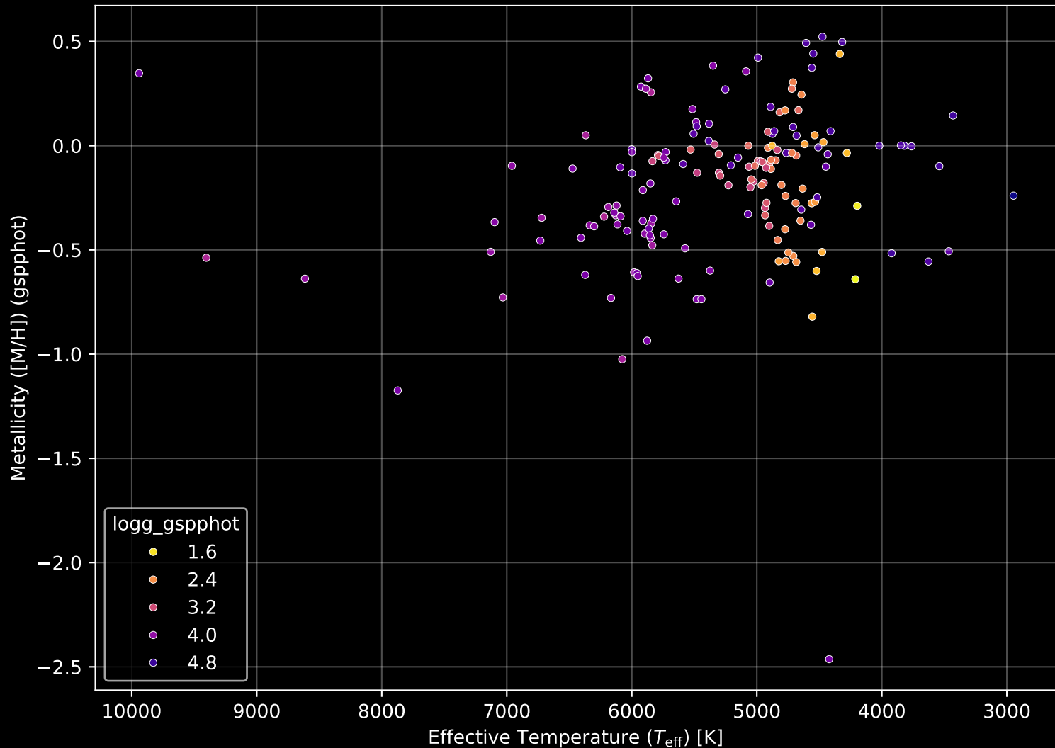
APOGEE DR17 Field: [273-24-O_TESS] Stellar Population Parameters (n= 169)
