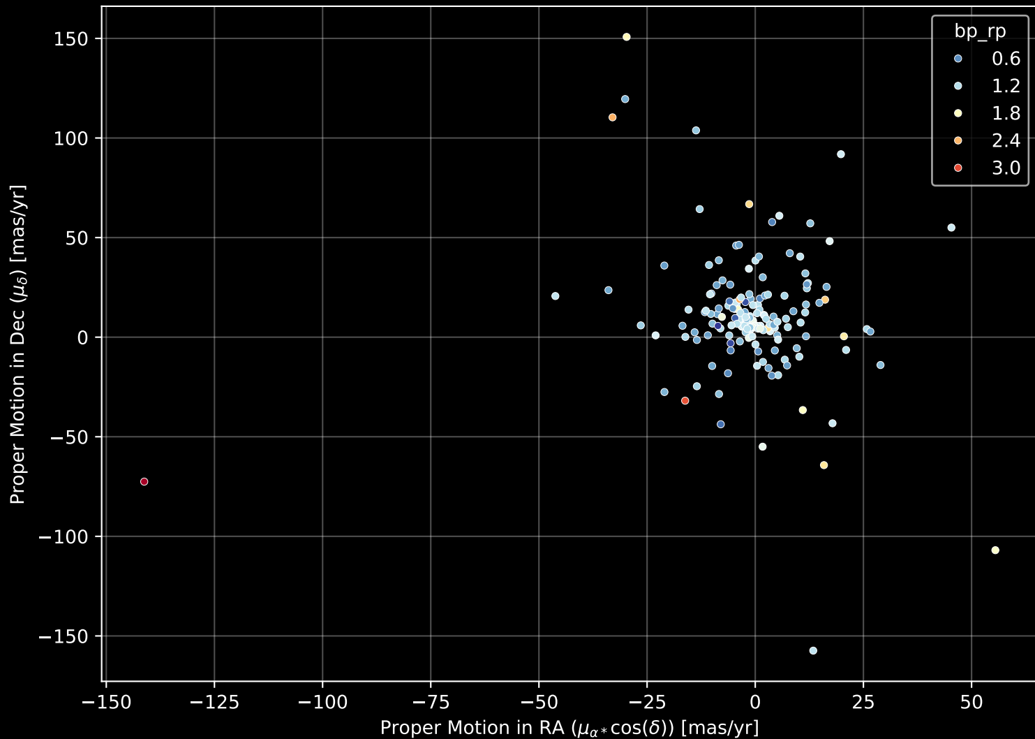
APOGEE DR17 Field: [273-24-O_TESS] Proper Motion Diagram (n= 169)
