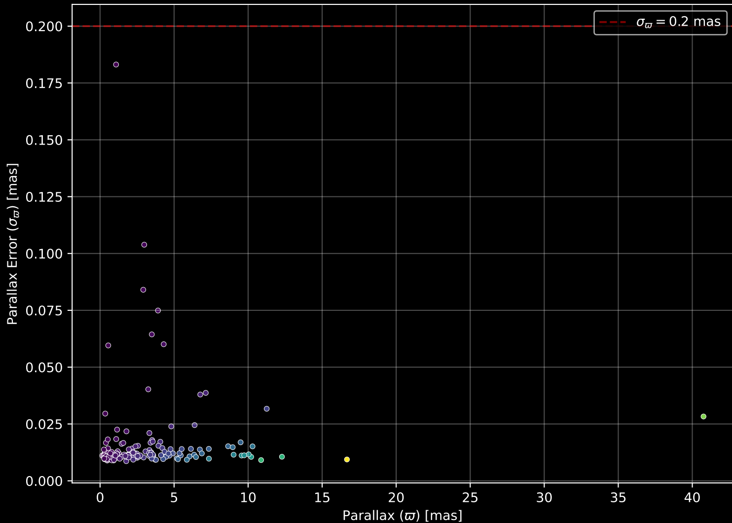
APOGEE DR17 Field: [273-24-O_TESS] Parallax Quality (n= 169)
