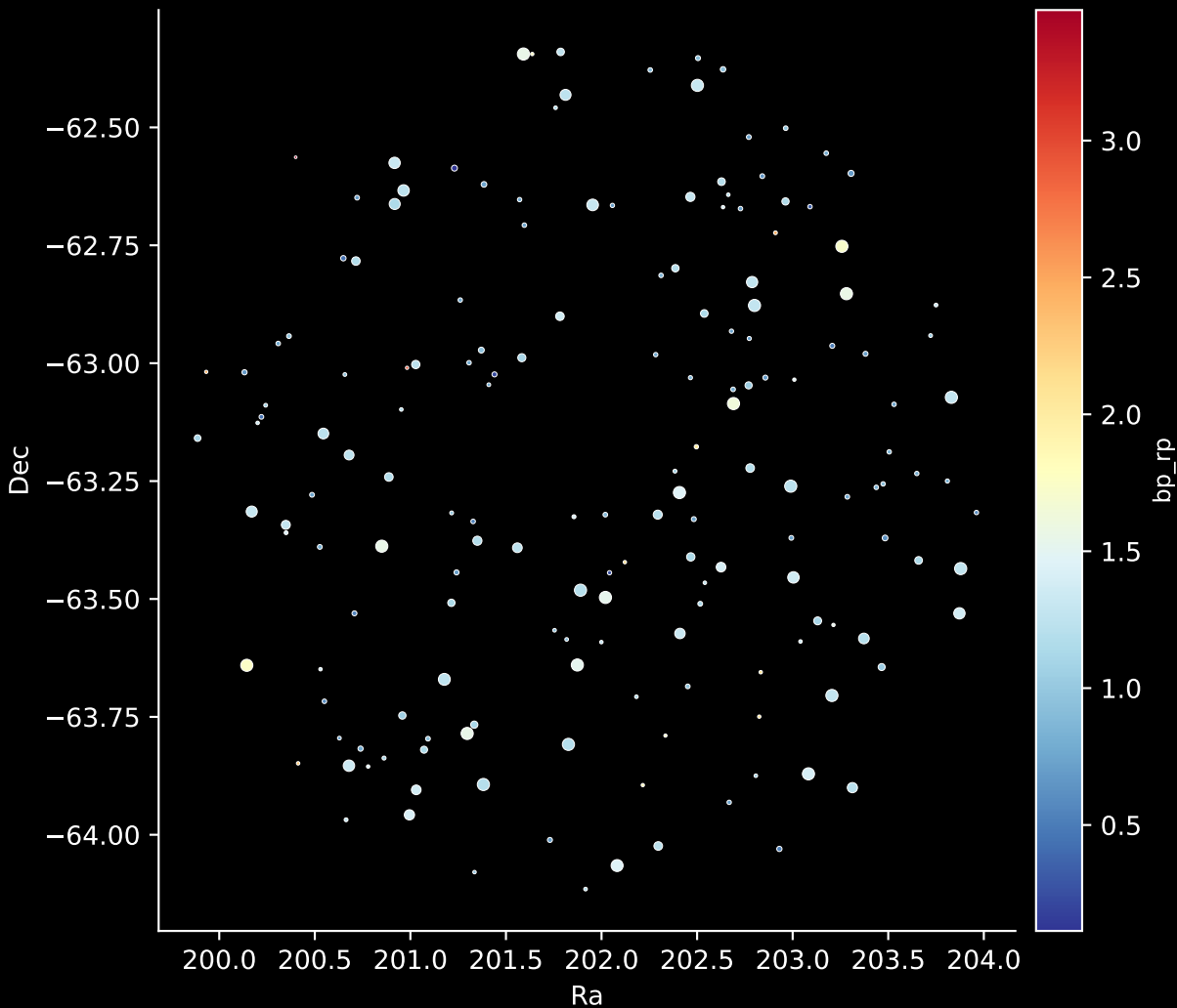
APOGEE DR17 Field: [273-24-O_TESS] Stars: 169
